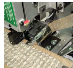
Bond Model PBB-2X applying 7/8" Veltron on a mat.
