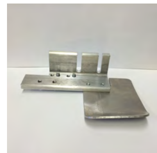
PBB Folder Bracket Sku #: PBB16001/2CP Fast & easy way to switch between folder sizes. Used for mounting any PBB folders- complete with bracket, guide plate and screws
