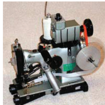
Model HDP-2 Heavy Duty Portable (STK#21405) Our TMB table model head is converted to be the most heavy duty portable available. Lock stitch bobbin machine with double pullers and speed control. Designed for workrooms in mind (weighs 70 lbs).
