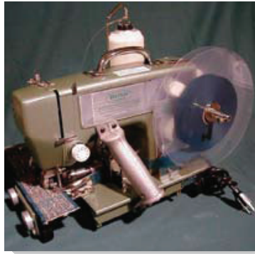
Model PBL-IX Single Puller Portable Carpet Binder (STK#21101X) Industry standard, built to last. Binds up to 3" width in a single pass with optional attachments. Fully adjustable zigzag to straight stitch with the turn of a knob. Four caster wheels and two float wheels for stability and ease of operation.
