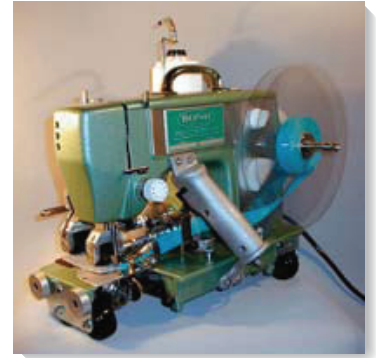
Model PBL-2X Double Puller Portable Carpet Binder (STK#21102X) Two clutches and puller wheels along with four caster and two float wheels make this the "four wheel drive vehicle of choice" for binding your heavy plush and berber carpets. Independent lifting of rear puller for radius work.
